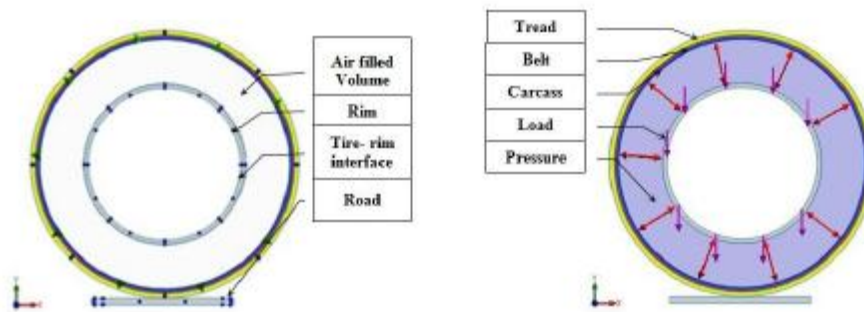
Fig4. Imposing of boundary conditions for radial tire.
